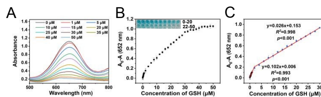
Fig. 4 (A) The UV absorption spectra of the colorimetric sensor with different concentrations of GSH (0–50 μM); (B) The absorbance difference of the sensor as a function of the GSH concentration, Inset: photographs of the sensor with different concentrations of GSH; (C) The linear correlations between the absorbance difference and the GSH concentration.
