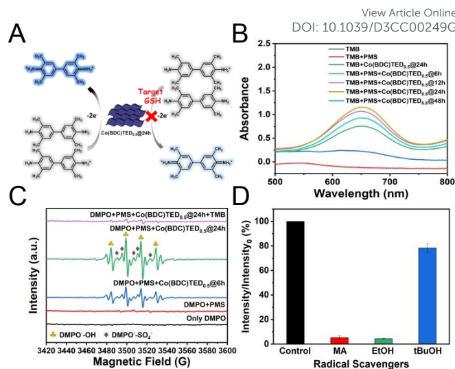
Fig. 2 (A) Schematic catalytic mechanism of Co(BDC)TED 0.5 as a catalyst. (B) UV-vis absorption spectra of different systems containing Co(BDC)TED 0.5 . (C) EPR spectra of PMS activation on Co(BDC)TED 0.5 under different conditions with DMPO. (D) Inhibitory effect of radical scavengers on TMB oxidation by PMS activation on Co(BDC)TED 0.5 @24h.
