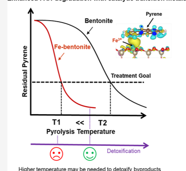
Enhanced PAH degradation with catalytic transition metals
